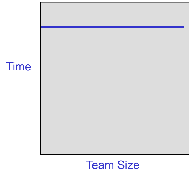
Non-Decomposable Task
